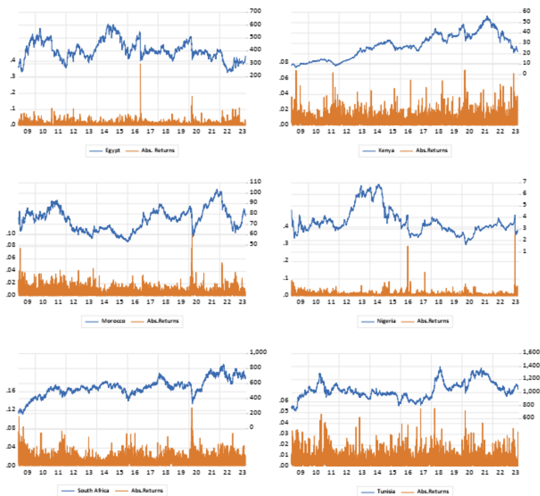
Figure 1. Plots of stock indices and absolute returns
