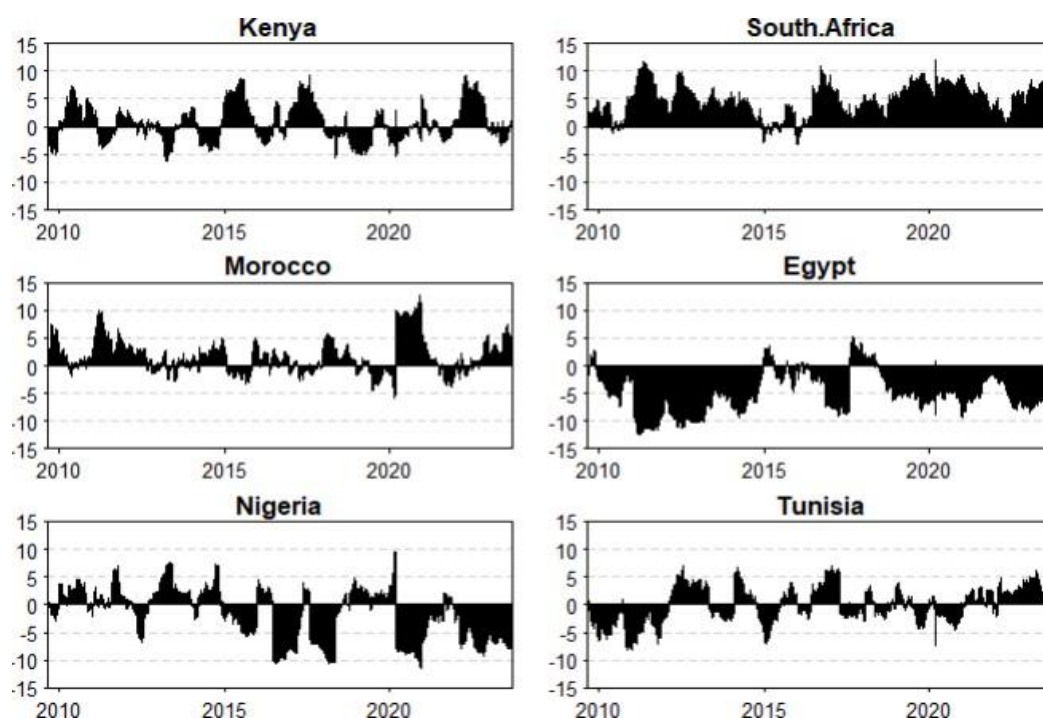
Figure 2. Net Total Directional Connectedness at the lower quantile
