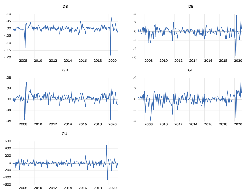
Figure 2. Return series
