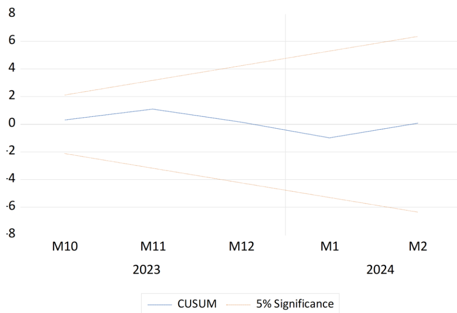
Figure 2. Cusum test for the FS2 model
